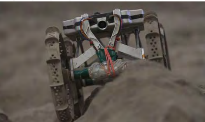
CubeRover Camera.
