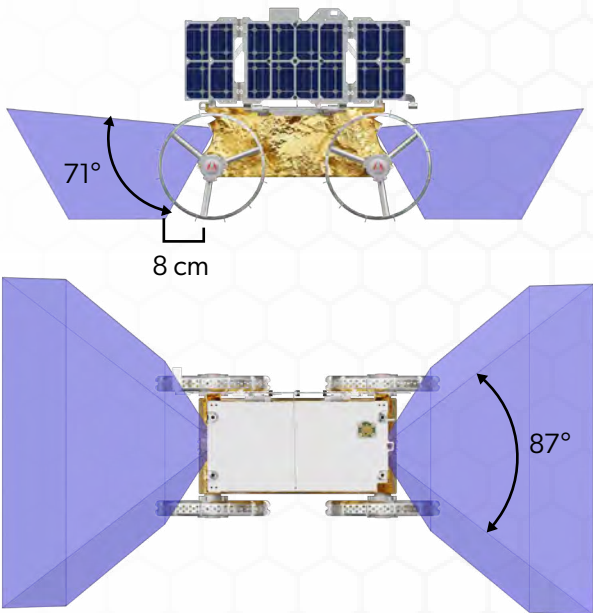
Camera vertical and horizontal fields of view.
